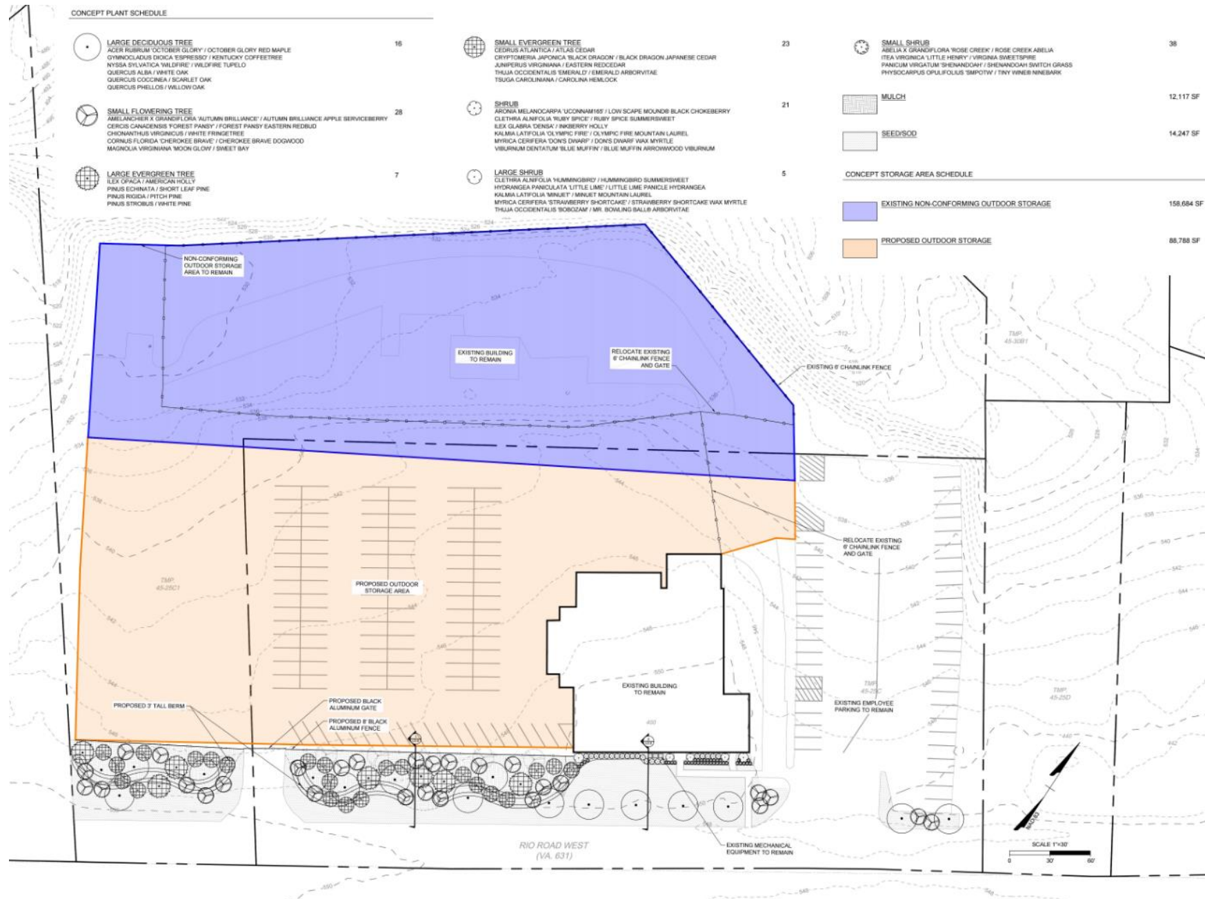
Figure 2: Proposed concept plan showing the buildings, travelways, outdoor storage, and parking.
